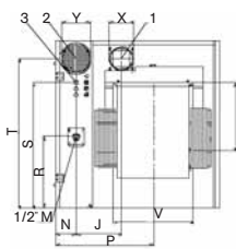
Back view M 20C - M 30C
