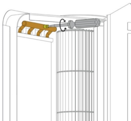
PIC. 17.2 BLEEDING/ AIR RELEASE VALVE.
