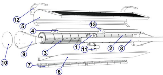
FIG. 3.1 CONSTRUCTION SLIM E.
